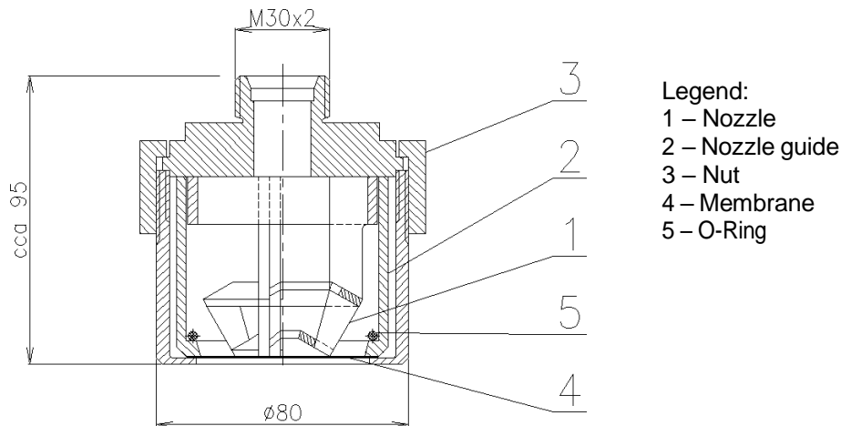
Figure No. 7 – DN 50 disc nozzle
